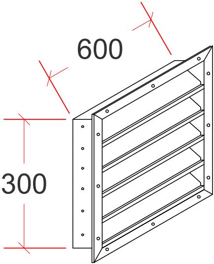
PERSPECTIVE VIEW
