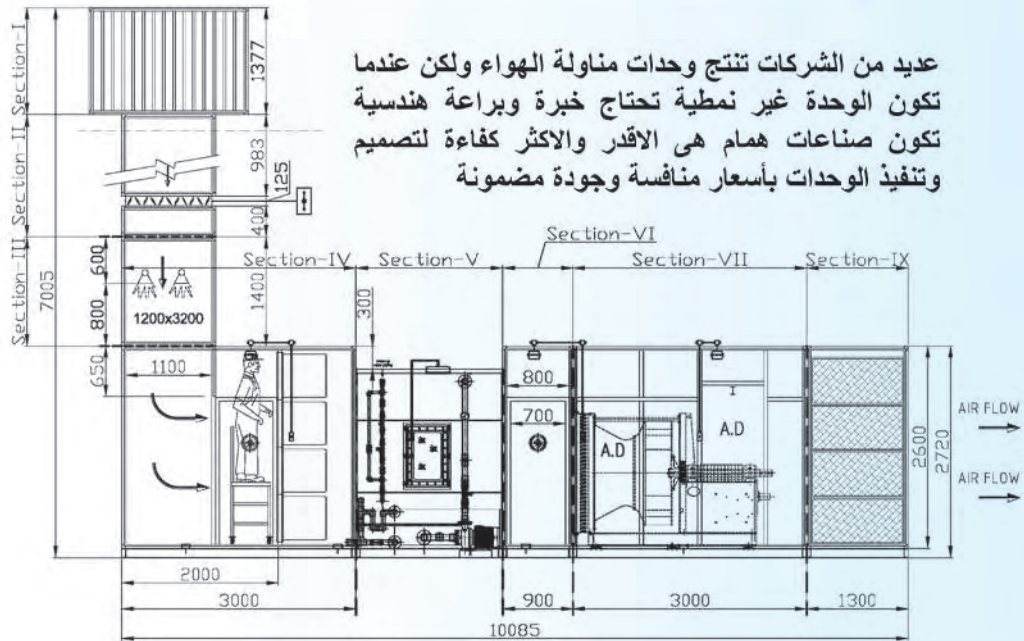
Air makeup unit for painting shops in car manufacturing
